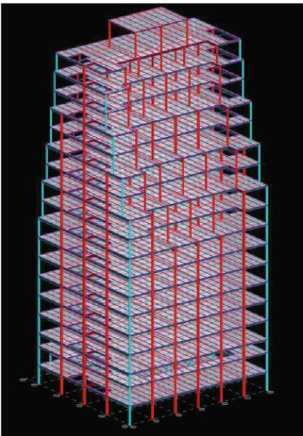
▲ Shmerykowsky Consulting Engineers' 3D model of Building 227.
